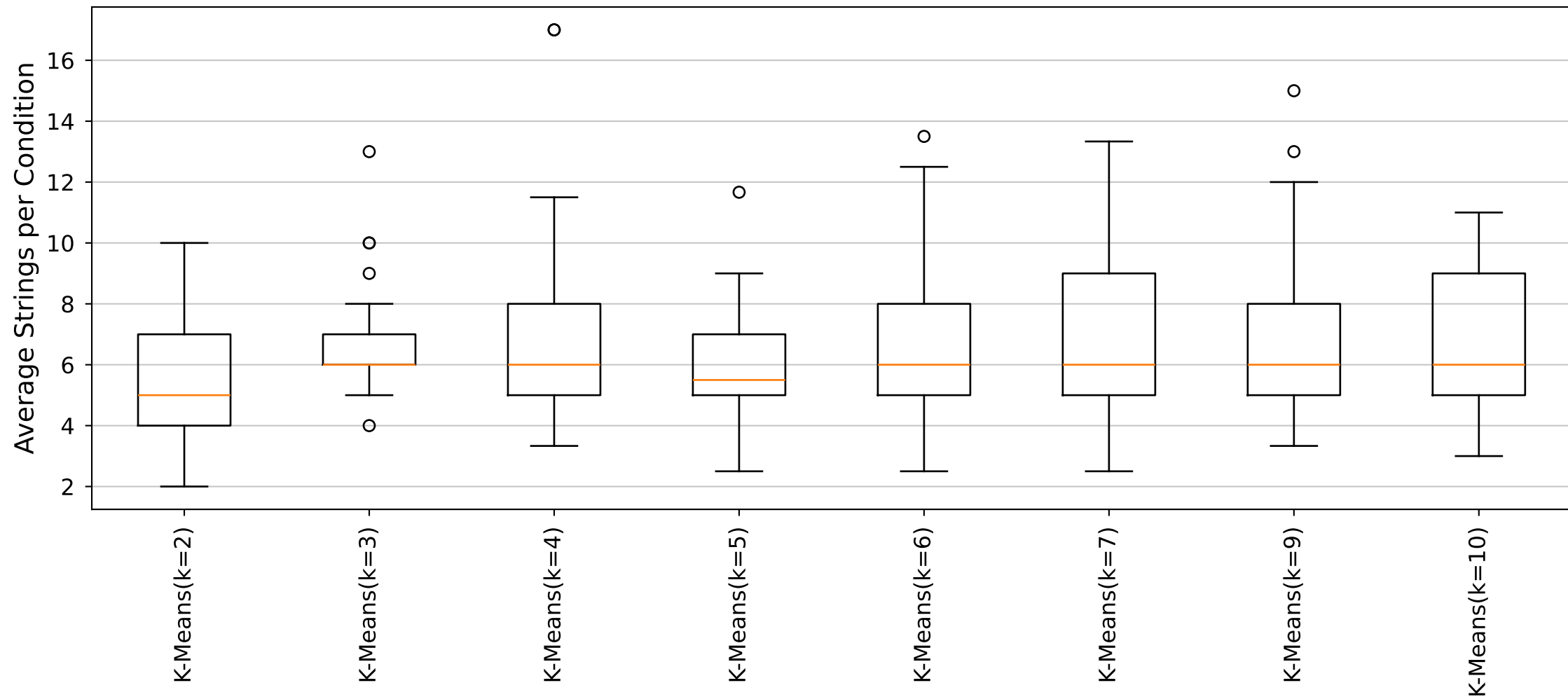
YARA Rules Average Strings per Condition Distribution (Cluster10_Size10 dataset)
